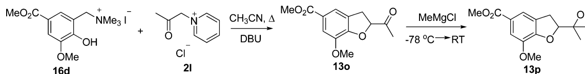
Scheme 19. Synthesis of Methyl ( \pm )-7-Methoxyanodendroate
