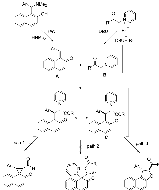
Scheme 10. Proposed Mechanism for the Formation of 1,2-Dihydronaphtho[2,1- b ]furans
