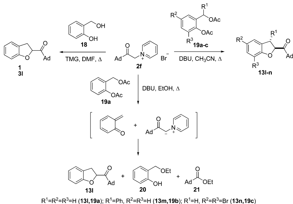
Scheme 18. Proposed Mechanism for the Generation of o -QMs from 2-Acetoxybenzyl Acetates
